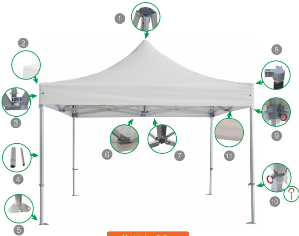
Model size: 3x3m Item No.: UT3350
